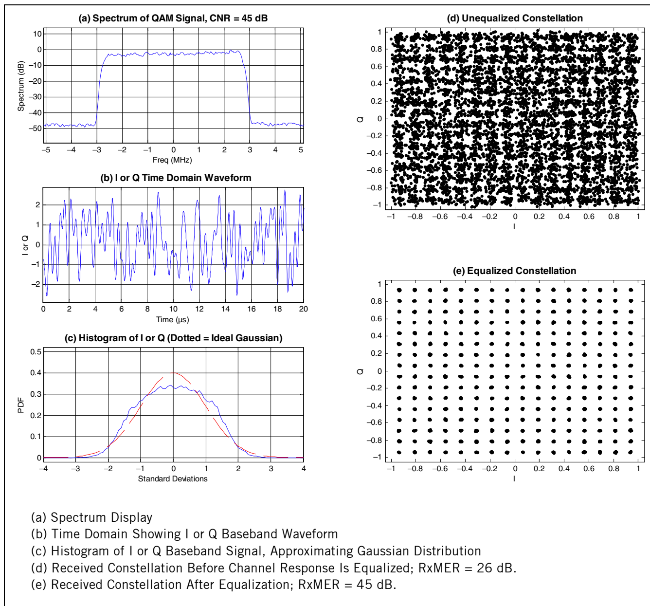
Figure 9: Views of a QAM Waveform (256 QAM, E_s/N_0 = 45 dB, with slight channel amplitude tilt and ripple)
